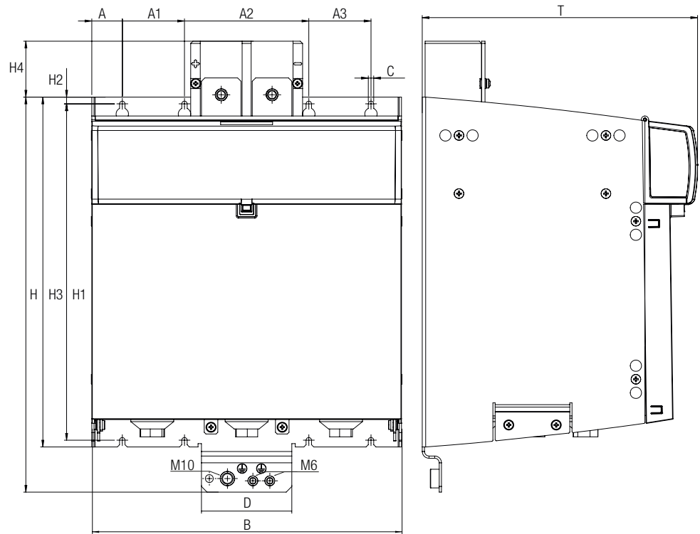
Figure 5.6 Dimensional sketches, KeDrive D3-ES energy storage
