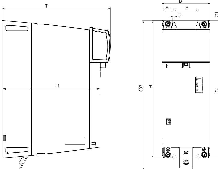
Figure 6.10 Dimensional drawing, D3-DC 300 module
