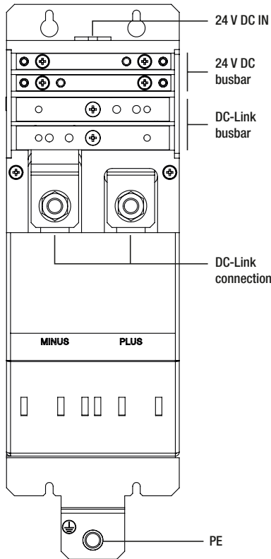
Figure 6.11 Connection module type D3-XV, connections
