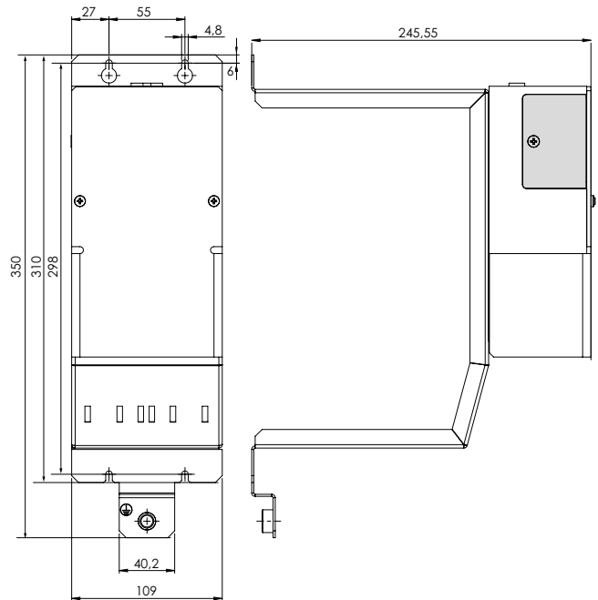
Figure 6.12 Connection module type D3-XV, dimensions
