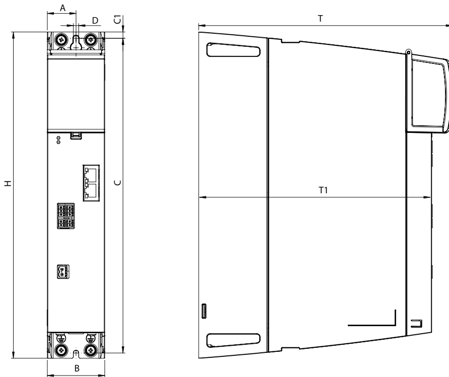
Figure 6.9 Dimensional drawing, D3-DE 300
