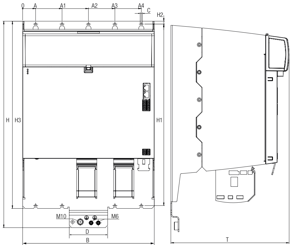
Figure 5.5 Dimensional sketches, KeDrive D3-EM energy manager
