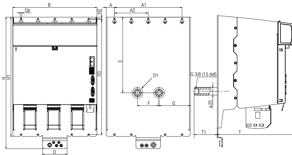
Figure 4.4 Dimensional drawings, KeDrive D3-DA BG4
