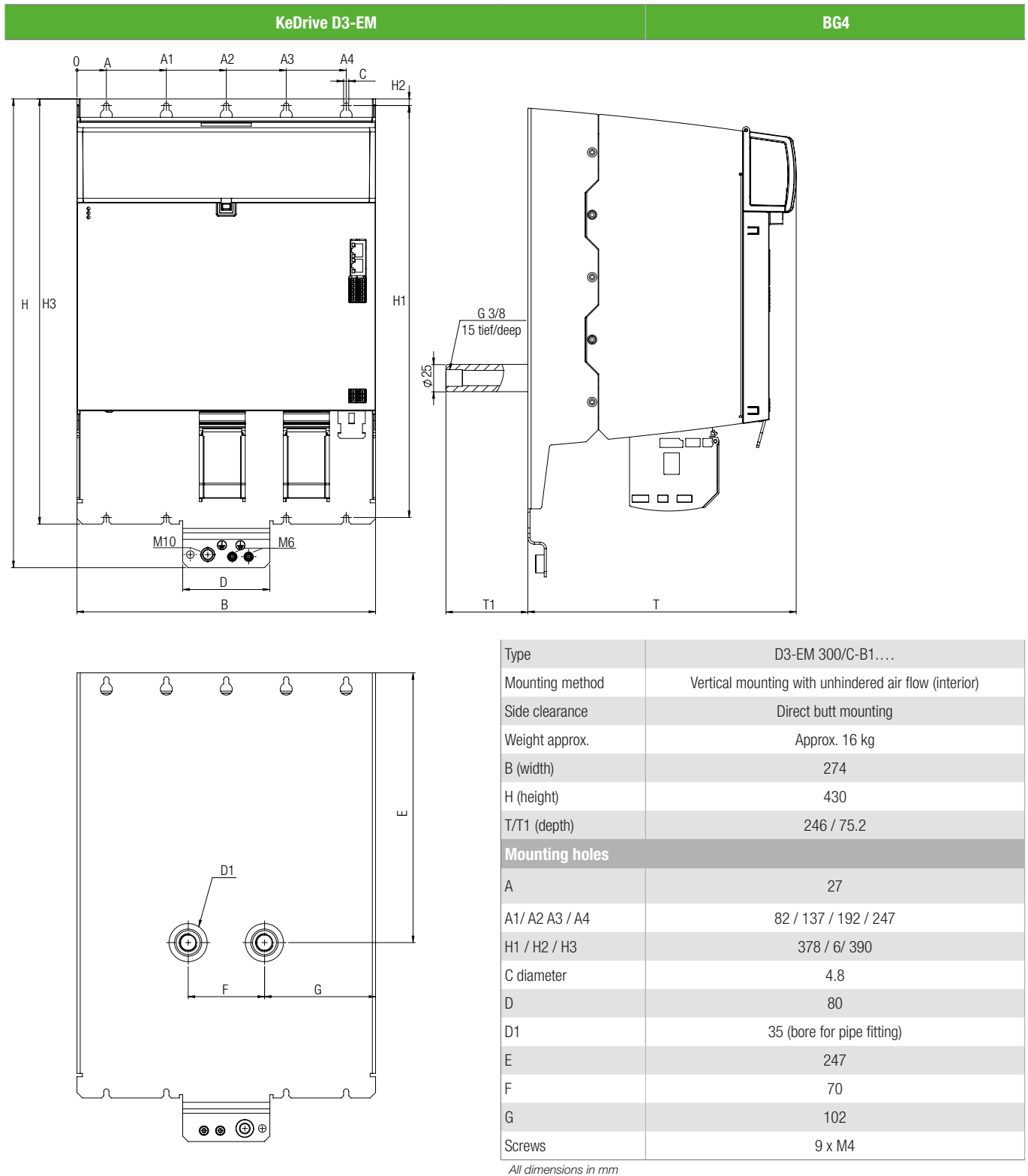
Figure 5.7 Dimensions, KeDrive D3-EM BG4 liquid cooling
